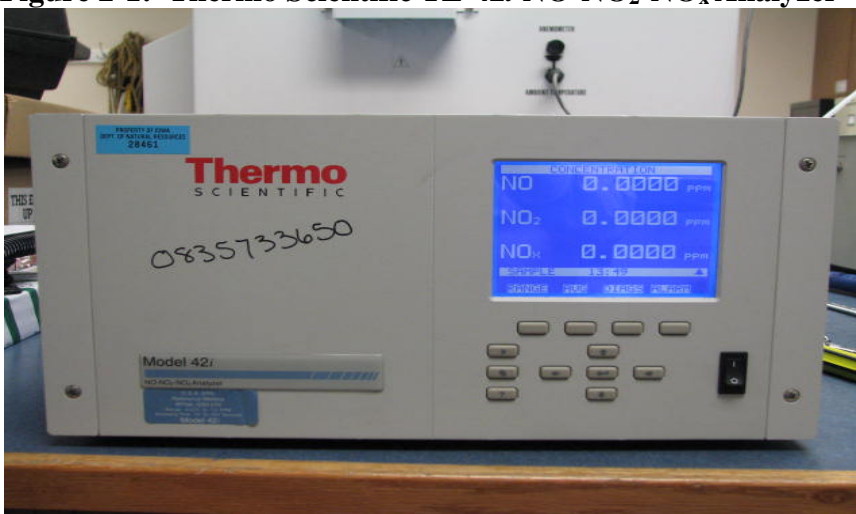
Figure 2-1: Thermo Scientific TL-42 i NO-NO 2 -NO x Analyzer
