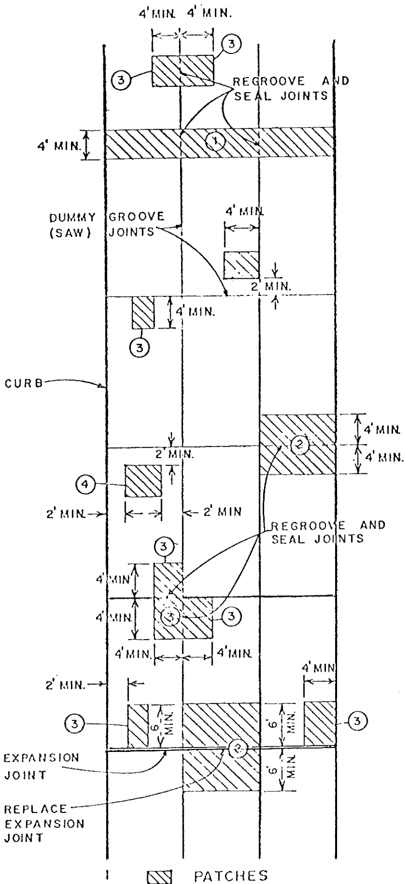
TYPICAL PATCH LOCATIONS FOR P.C.C. PAVEMENT
